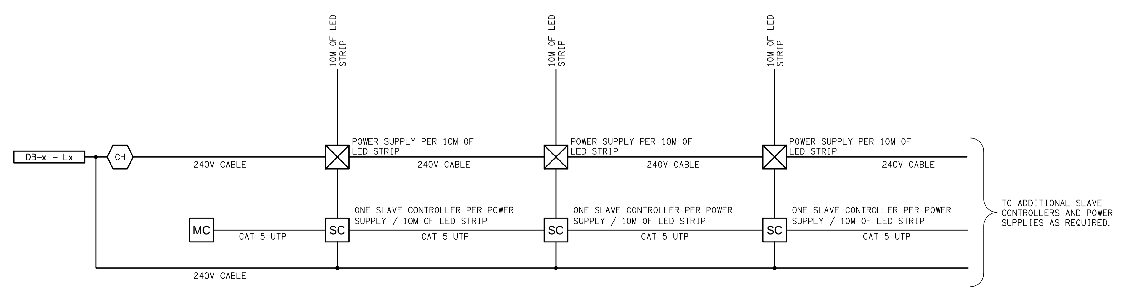
SCHEMATIC RGB CONTROL NOT TO SCALE
